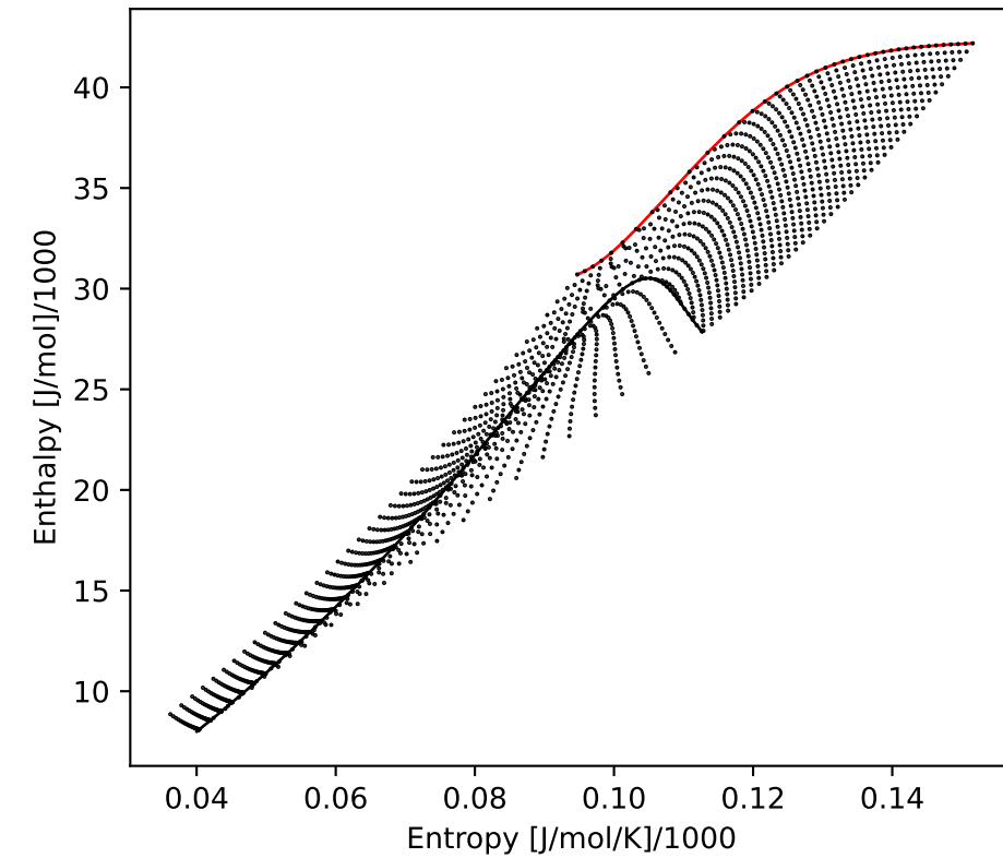
SmolarUmolar
