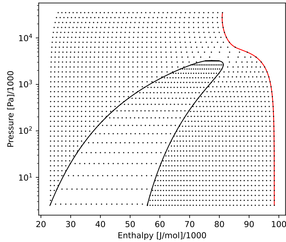
PUmolar
