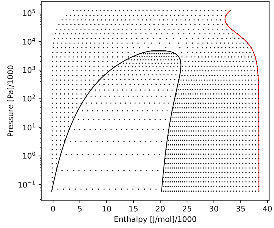
PUmolar
