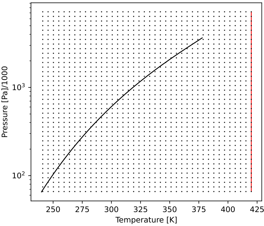
PSmolar
