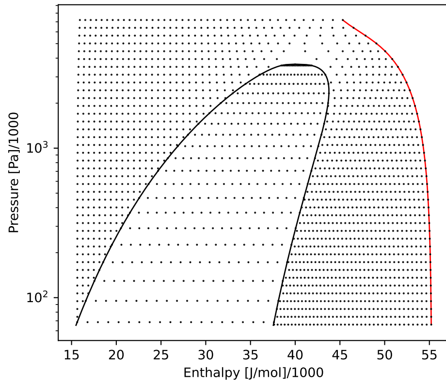
PUmolar
