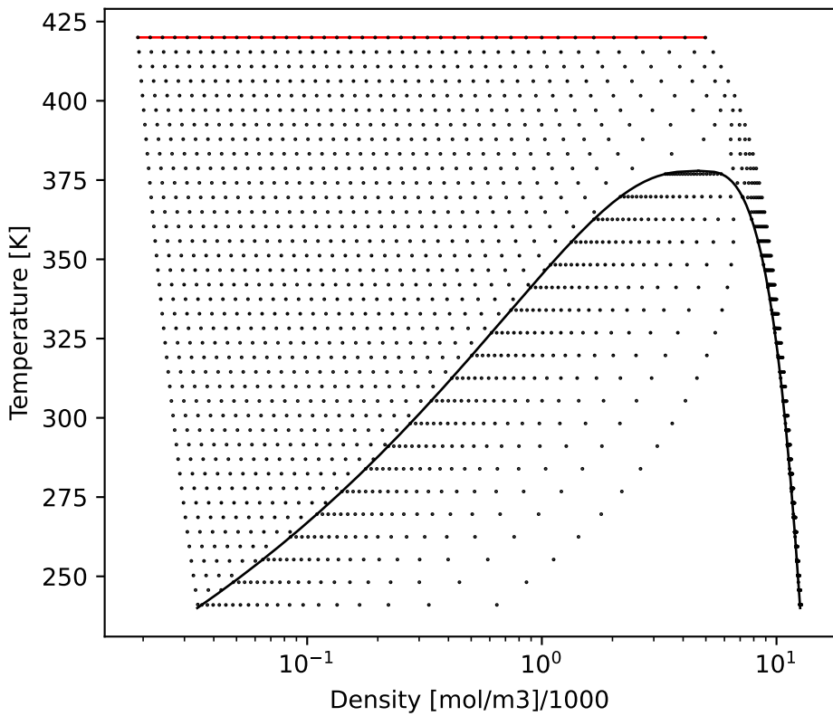
SmolarT
