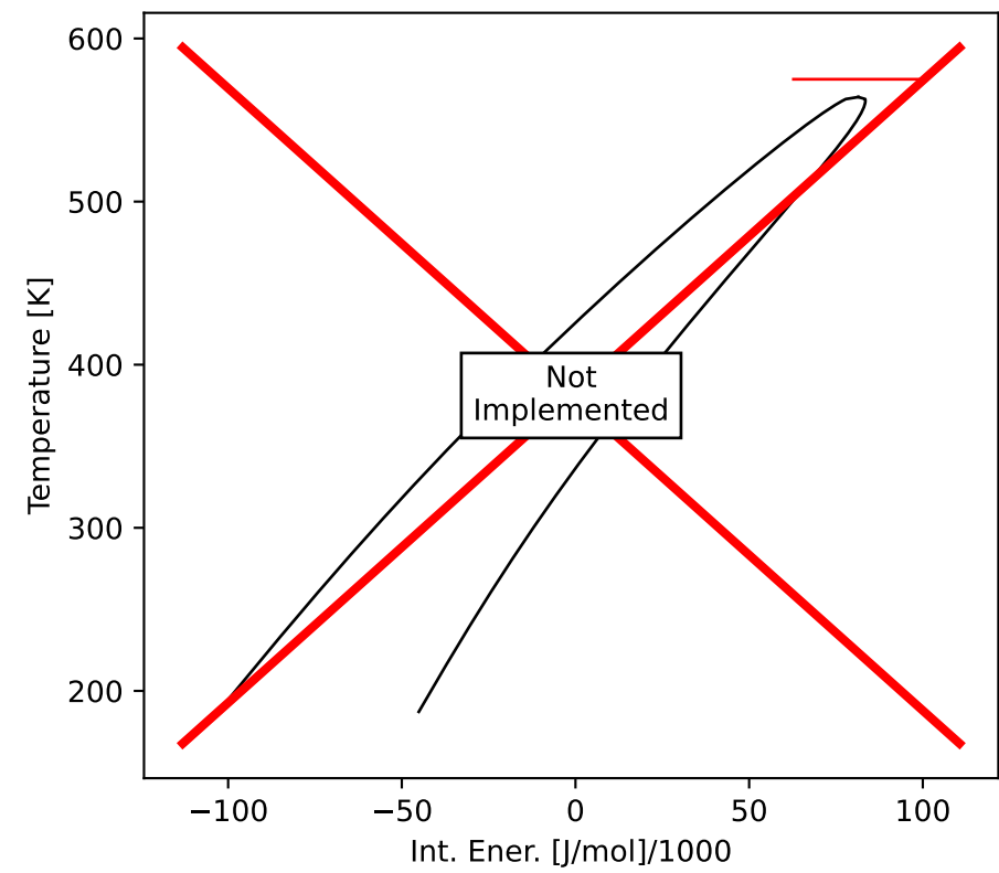
TUmolar
