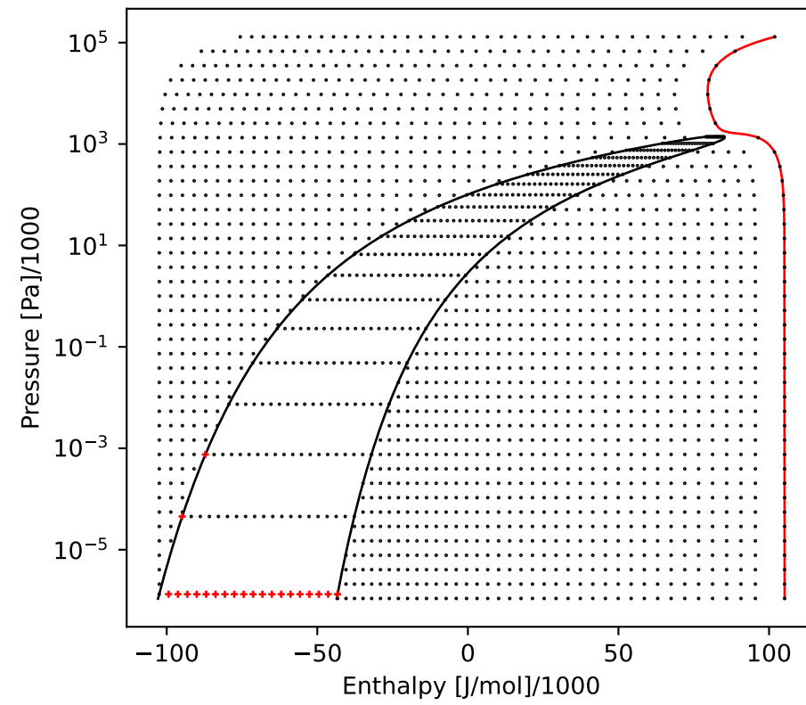
PUmolar
