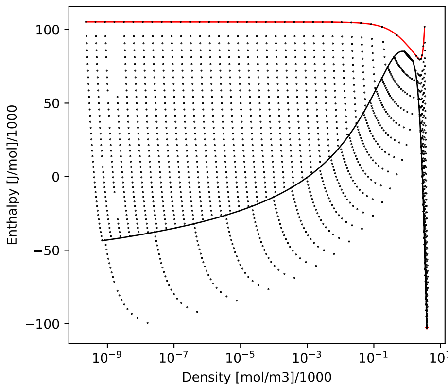
HmolarSmolar
