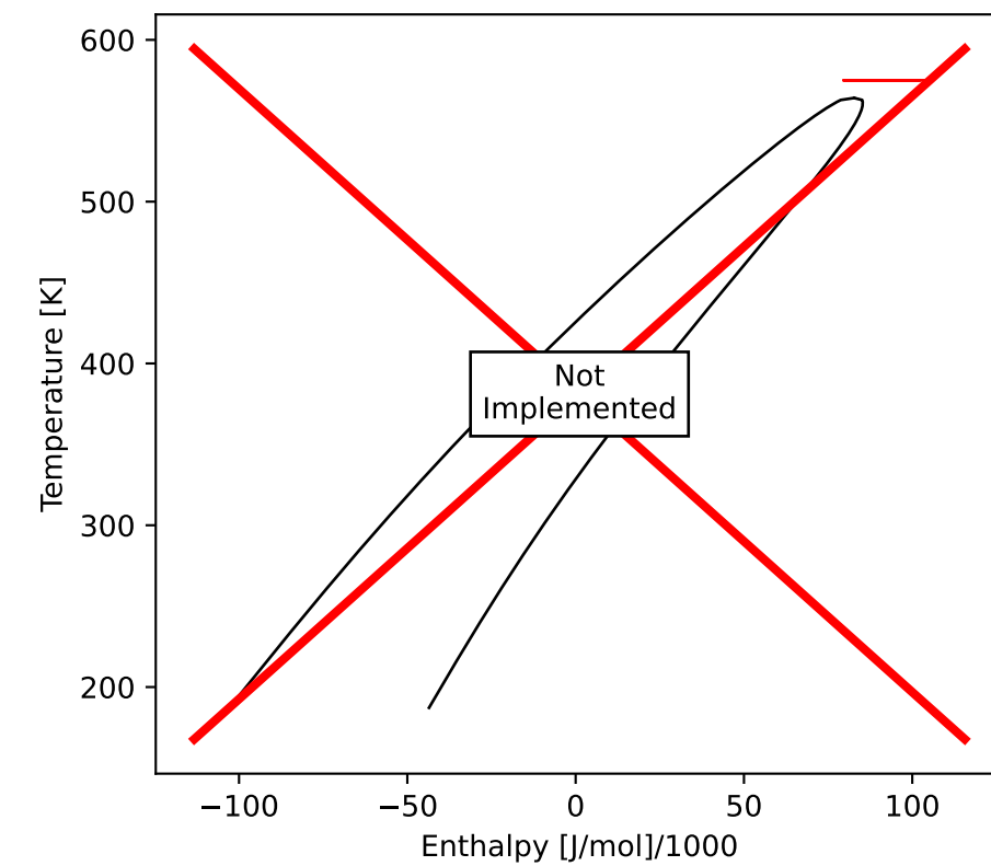
HmolarUmolar
