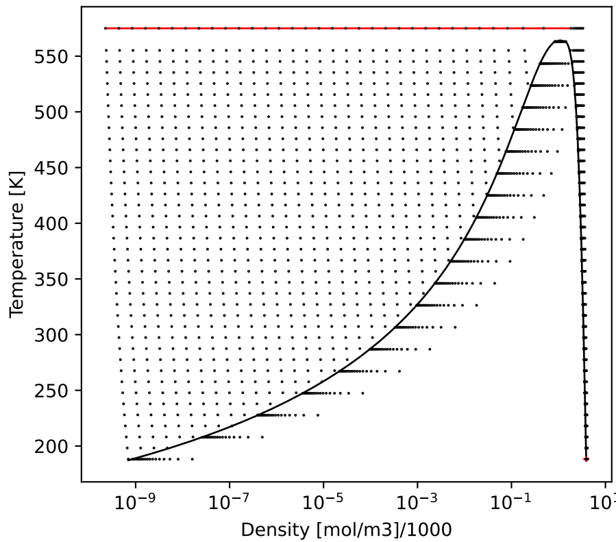
SmolarT
