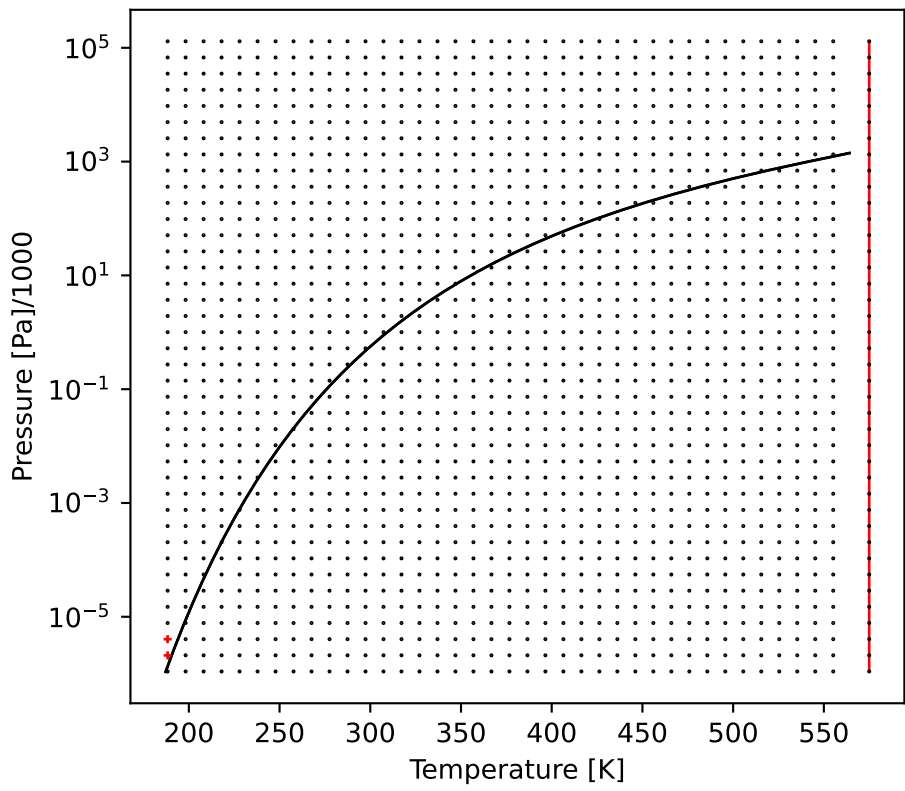
PSmolar
