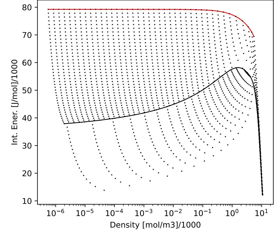
TUmolar
