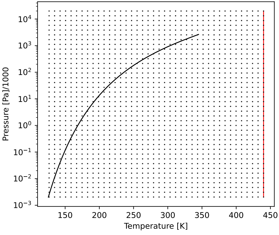
PSmolar
