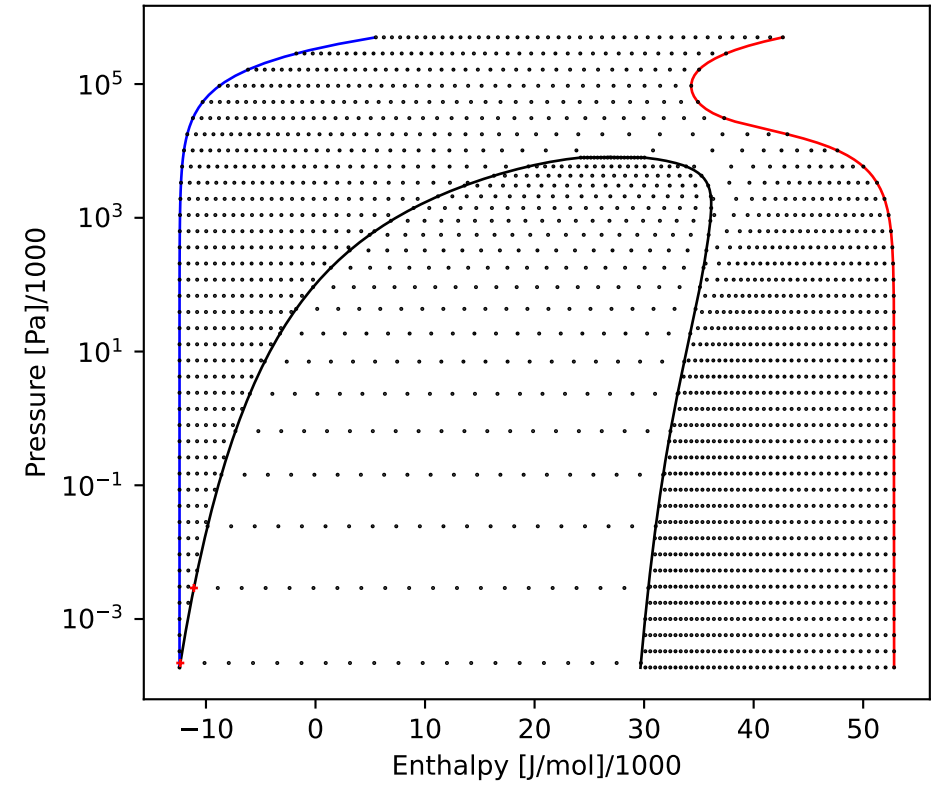
PUmolar
