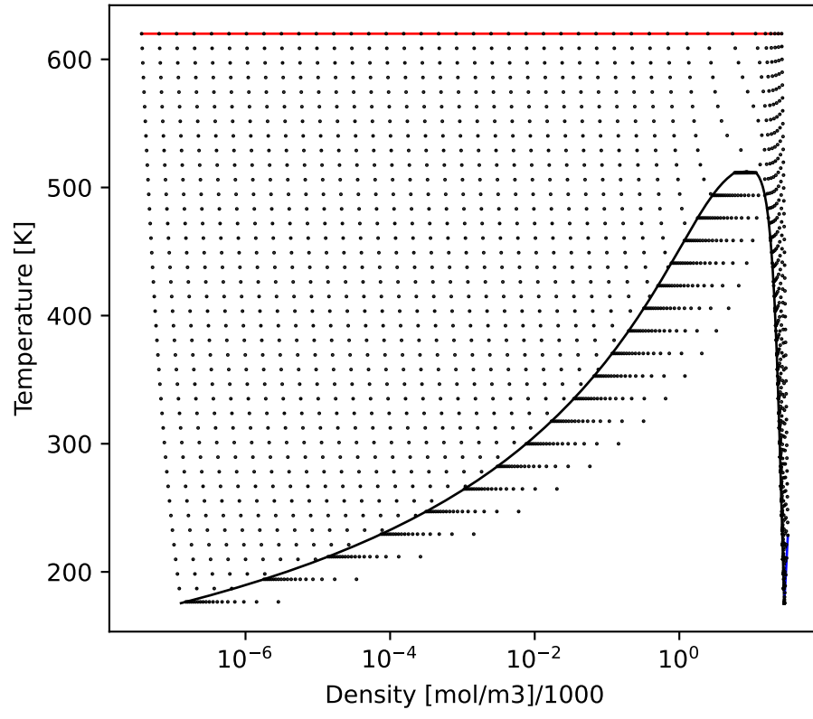
SmolarT
