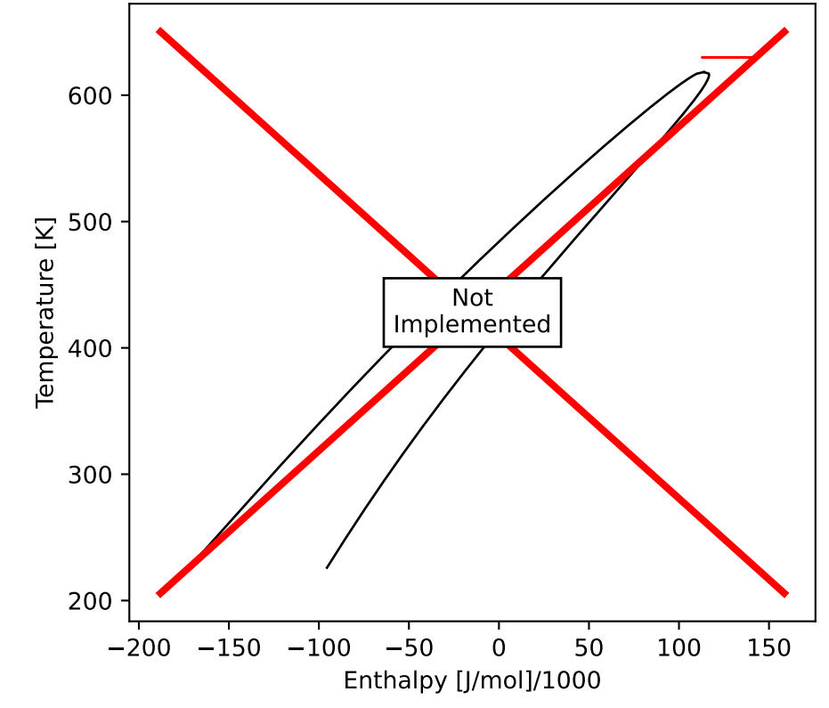
HmolarUmolar
