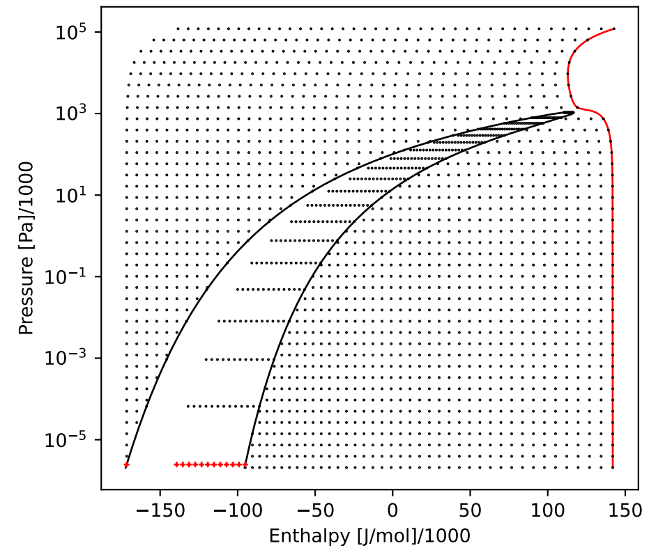
PUmolar
