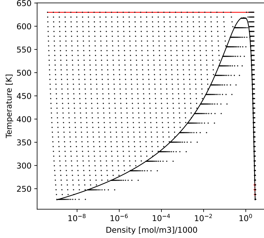
SmolarT
