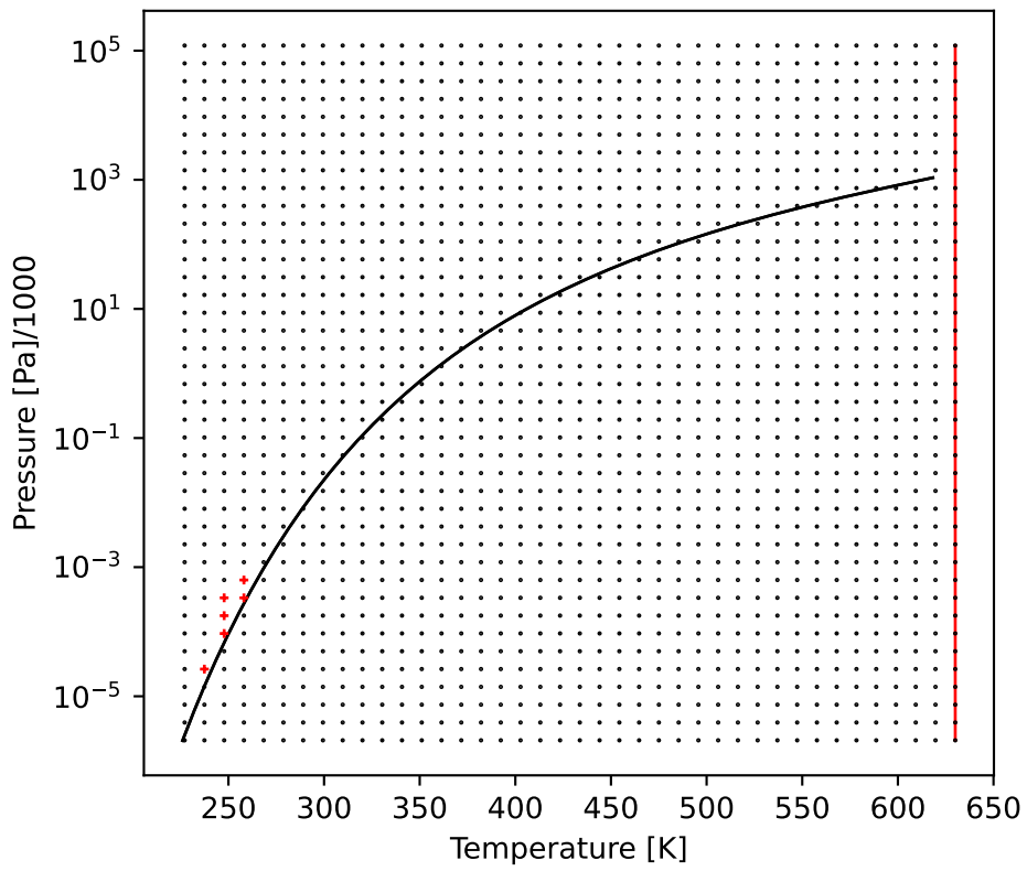
PSmolar
